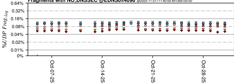
Fragments with NO_DNSSEC @EDNS0=4096 @2025-11-01T11:40:59.491369+00:00
