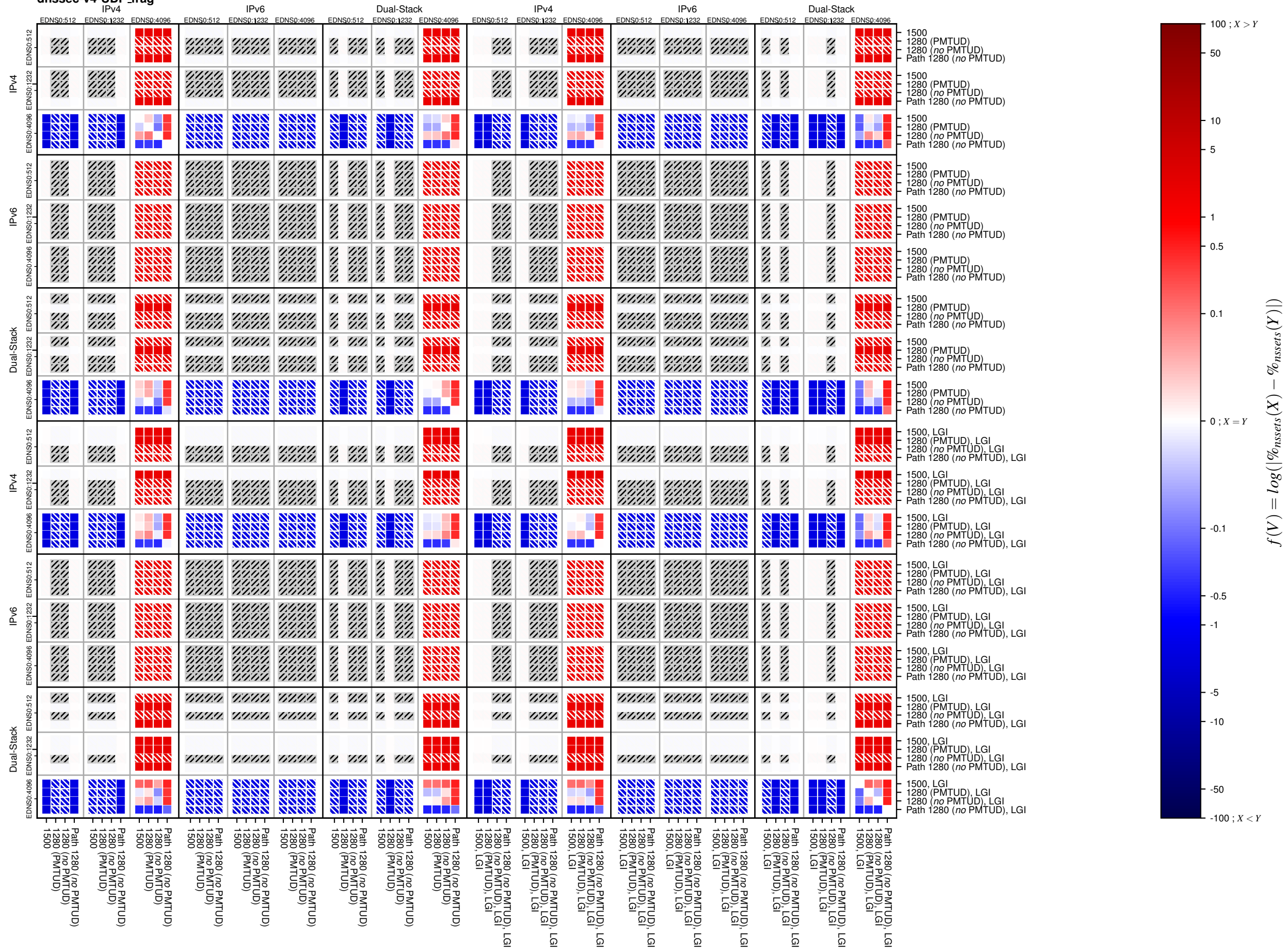
dnssec-v4-UDP_frag
