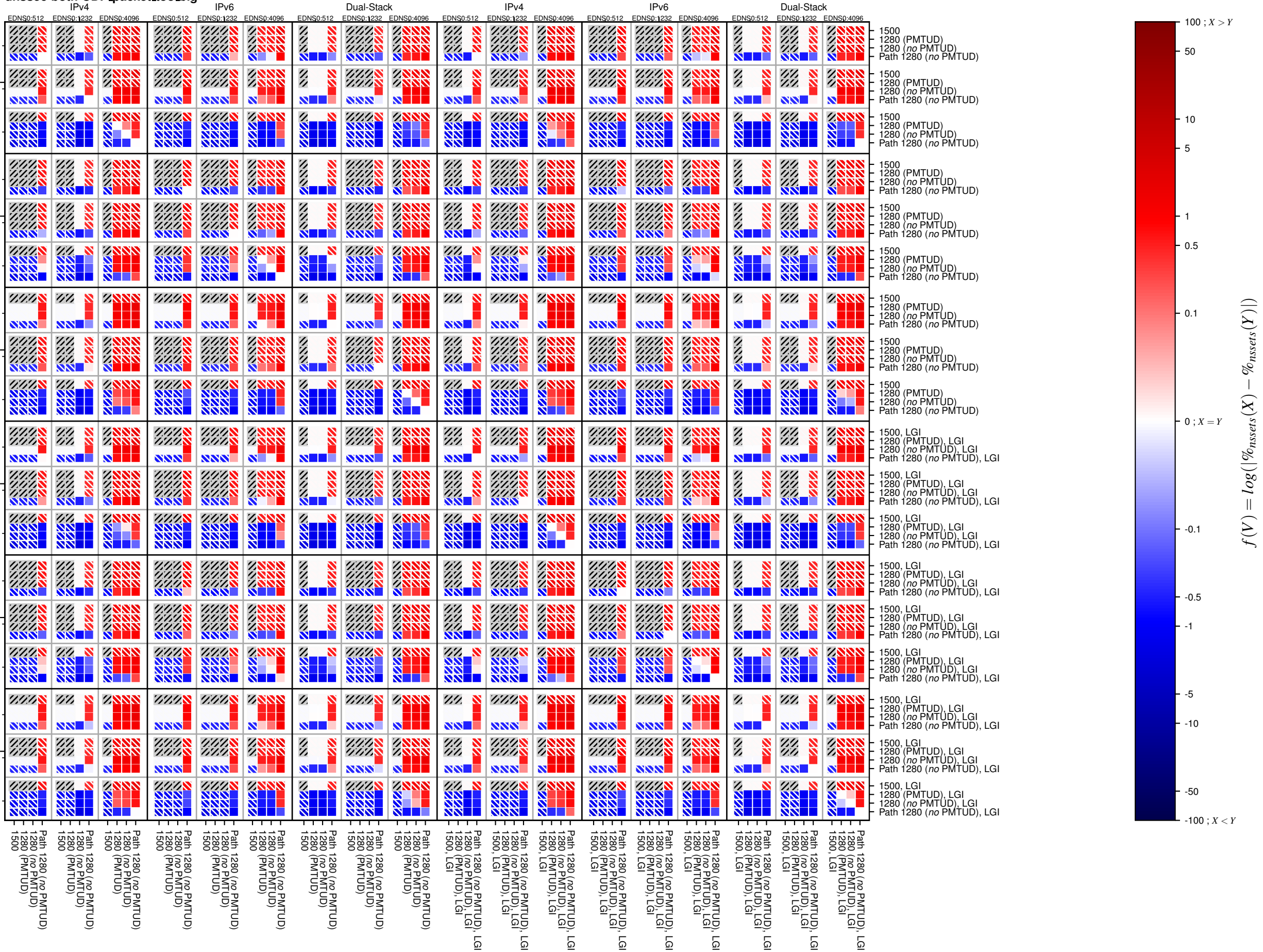
dnssec-both-UDP_packet_too_big
