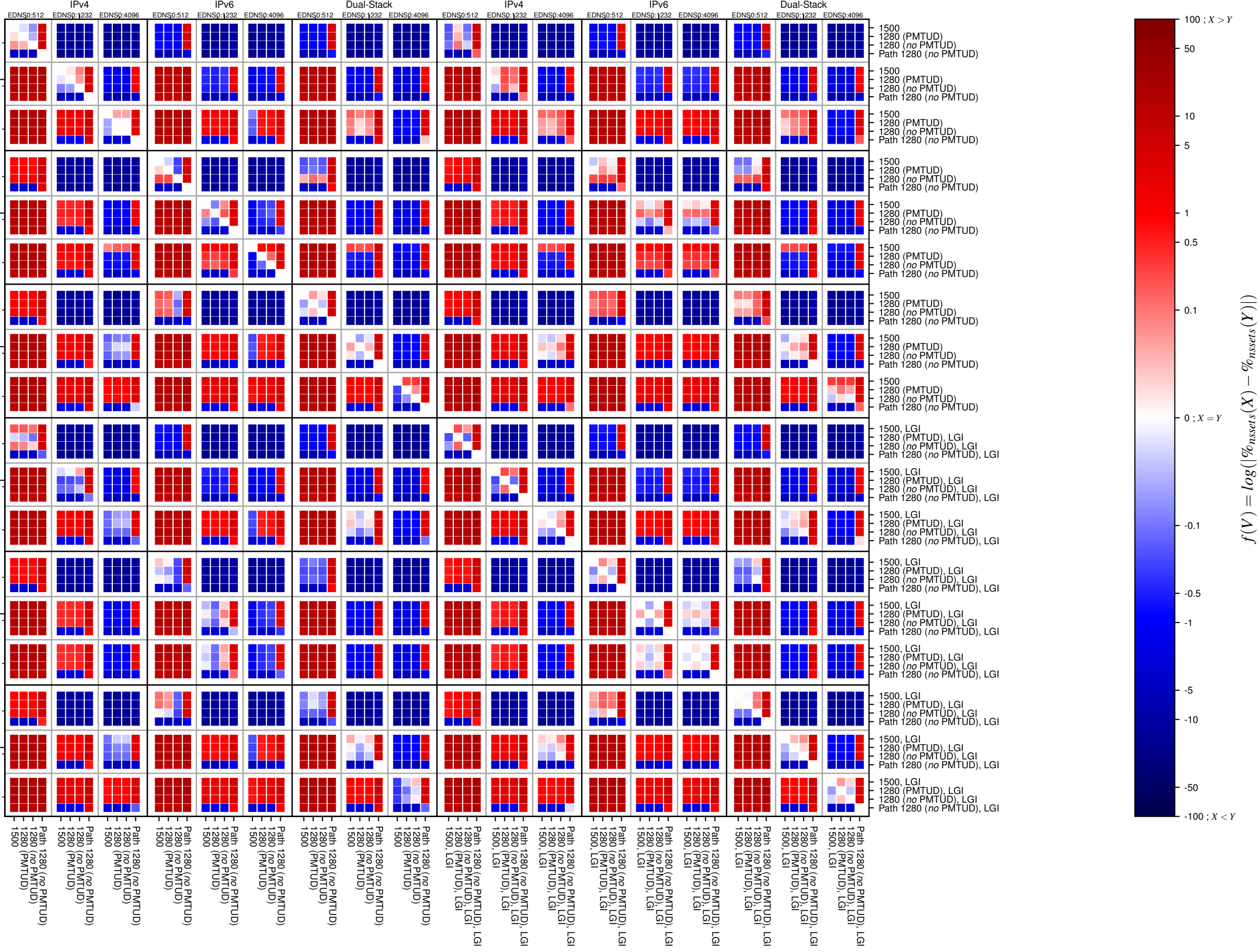
dnssec-both-TCP.count
