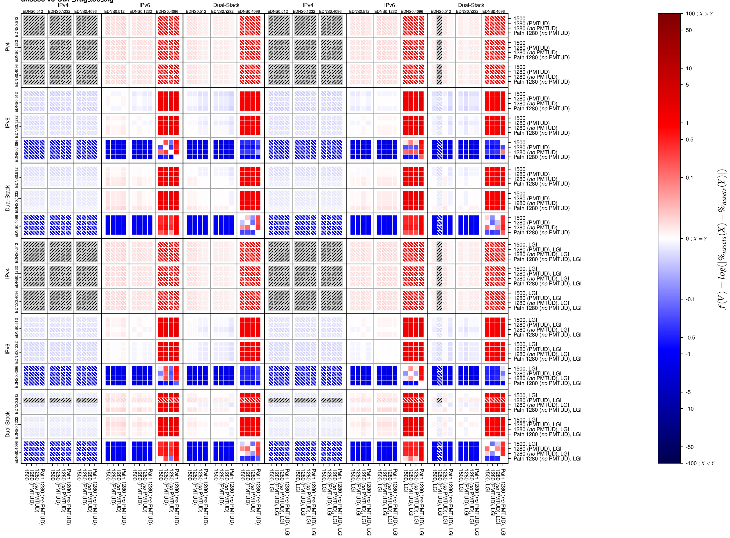
dnssec-v6-UDP_frag_too_big
