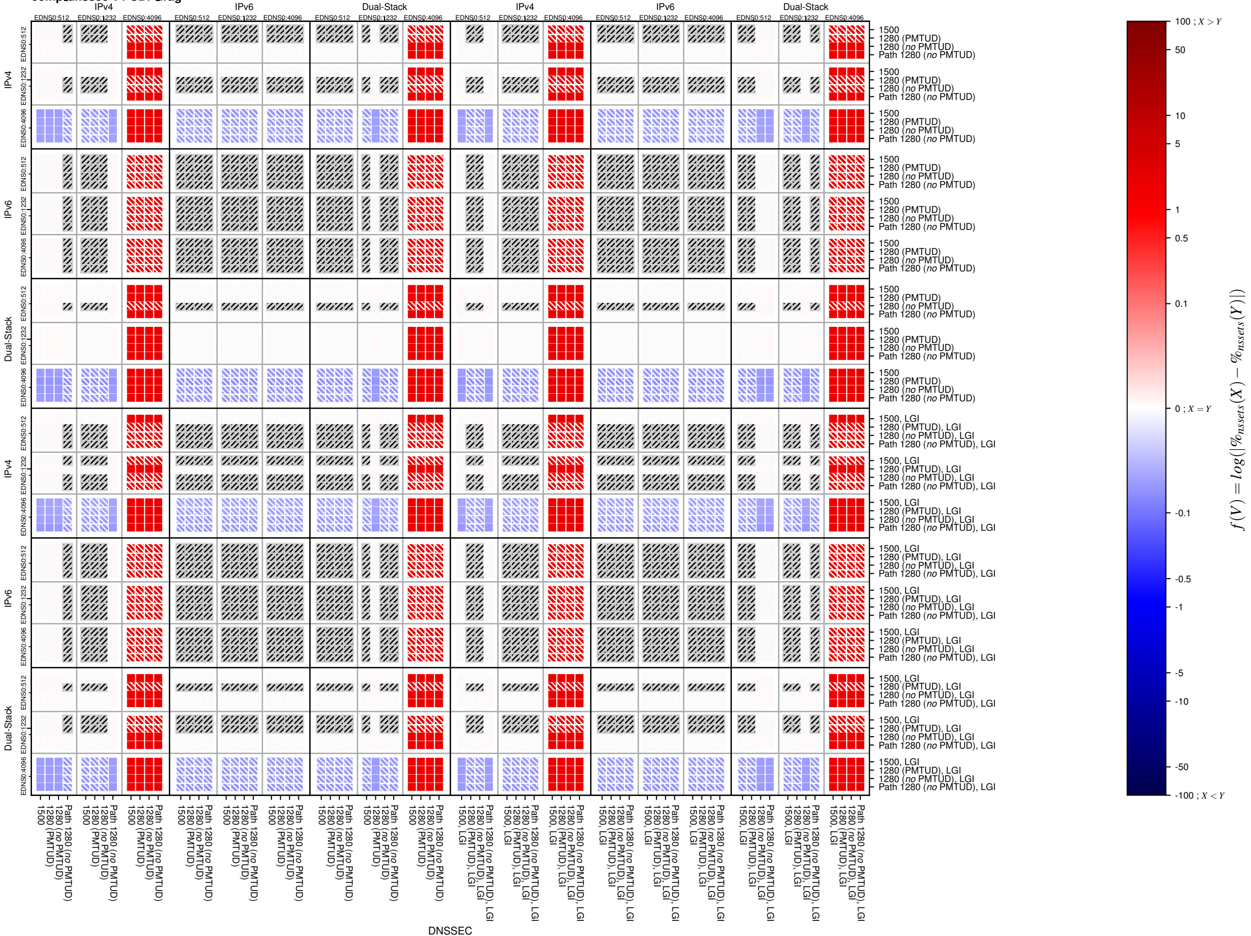
comp_dnssec-v4-UDP_frag
