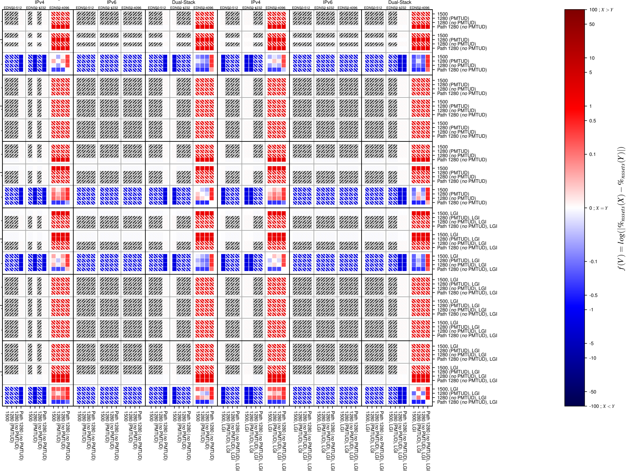
dnssec-v4-UDP_frag
