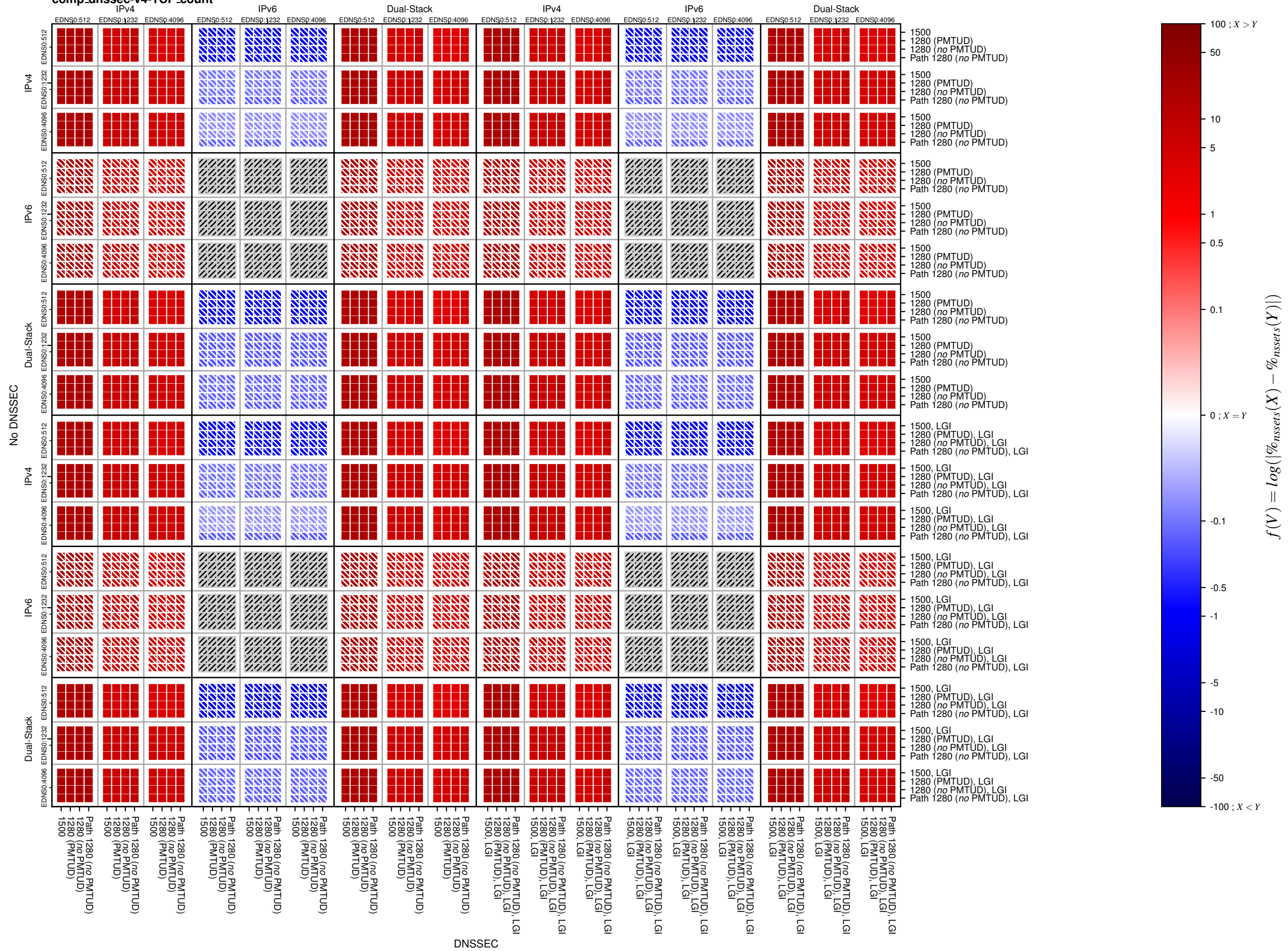
comp_dnssec-v4-TCP_count
