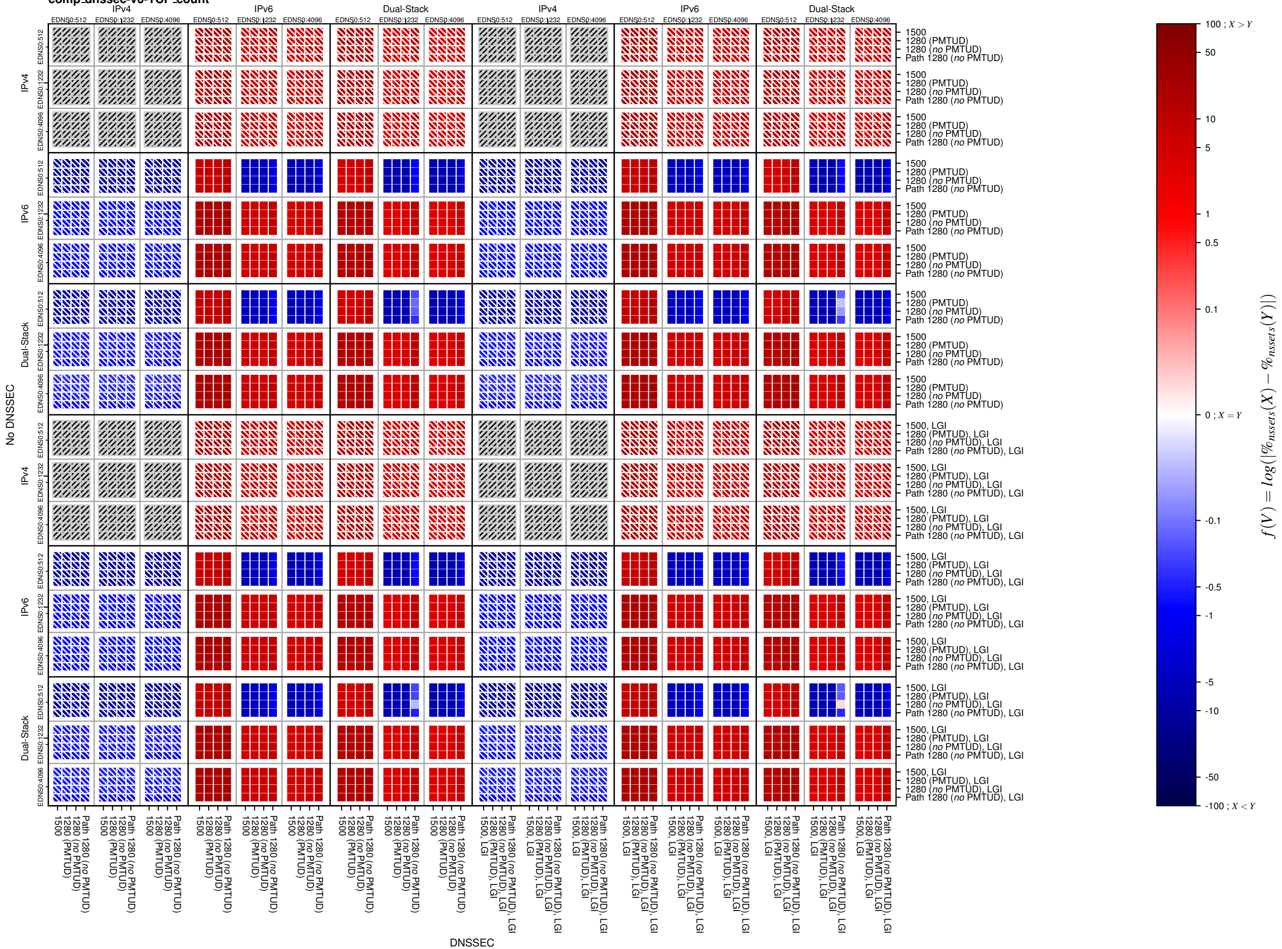
comp_dnssec-v6-TCP_count
