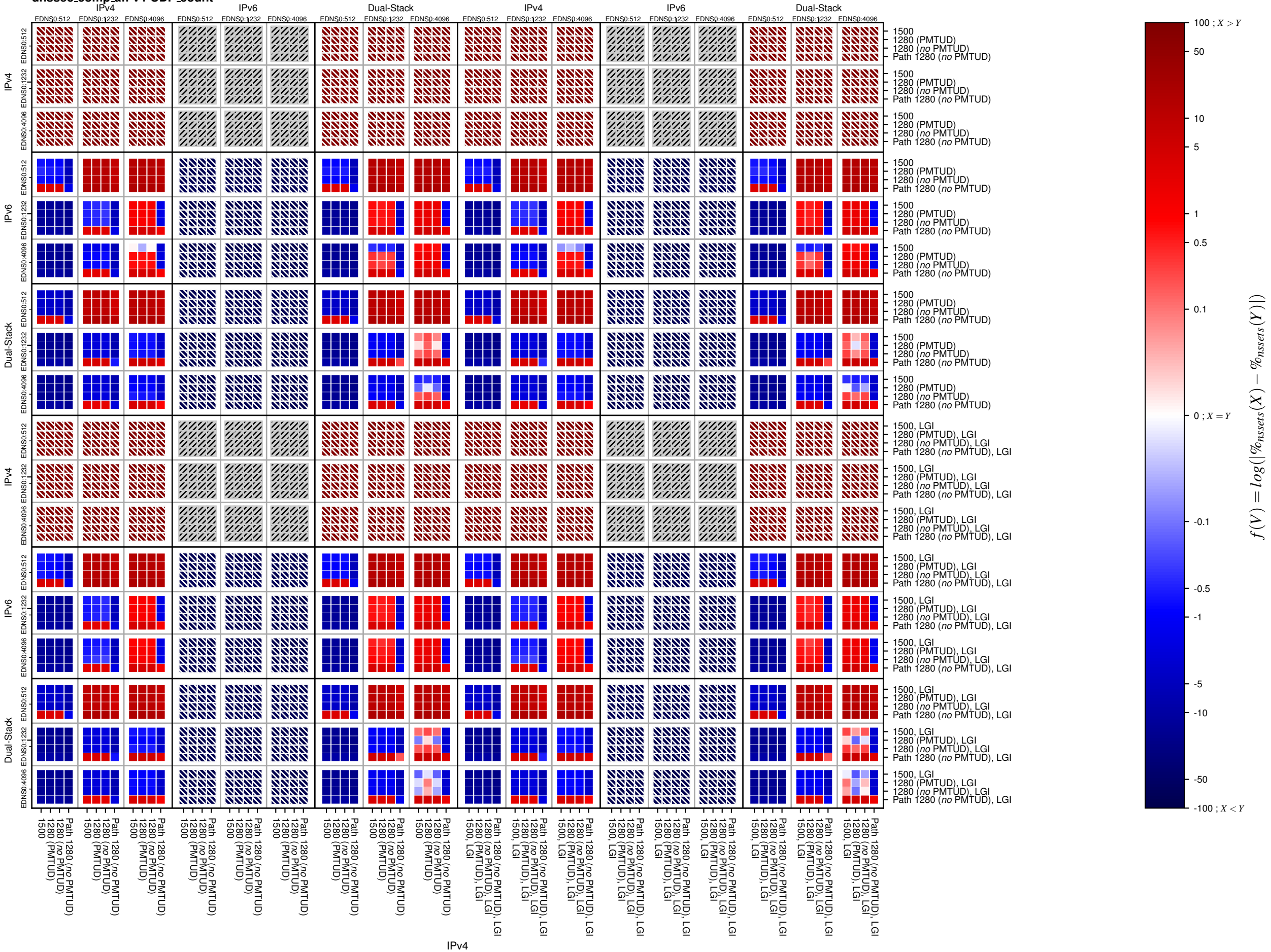
dnssec_comp_afv4-UDP_count
