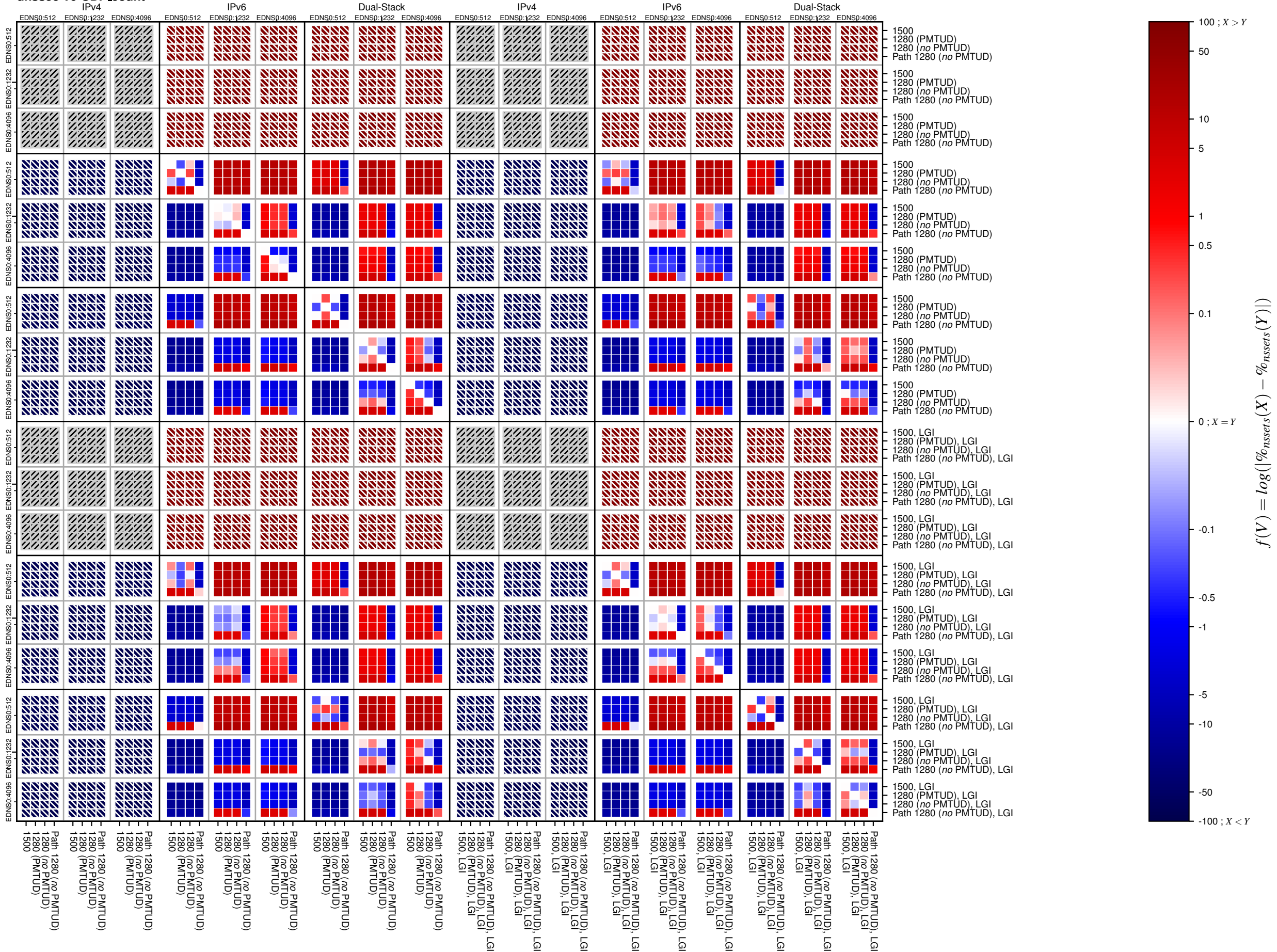
dnssec-v6-UDP_count
