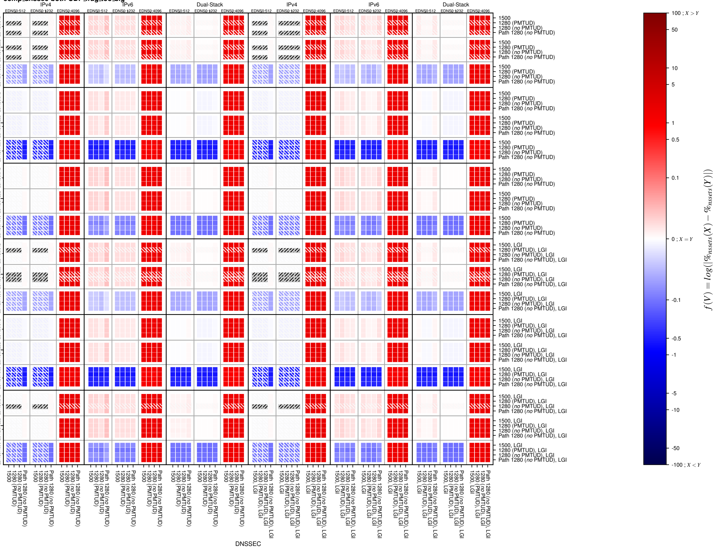
comp_dnsssec-both-UDP_frag_too_big
