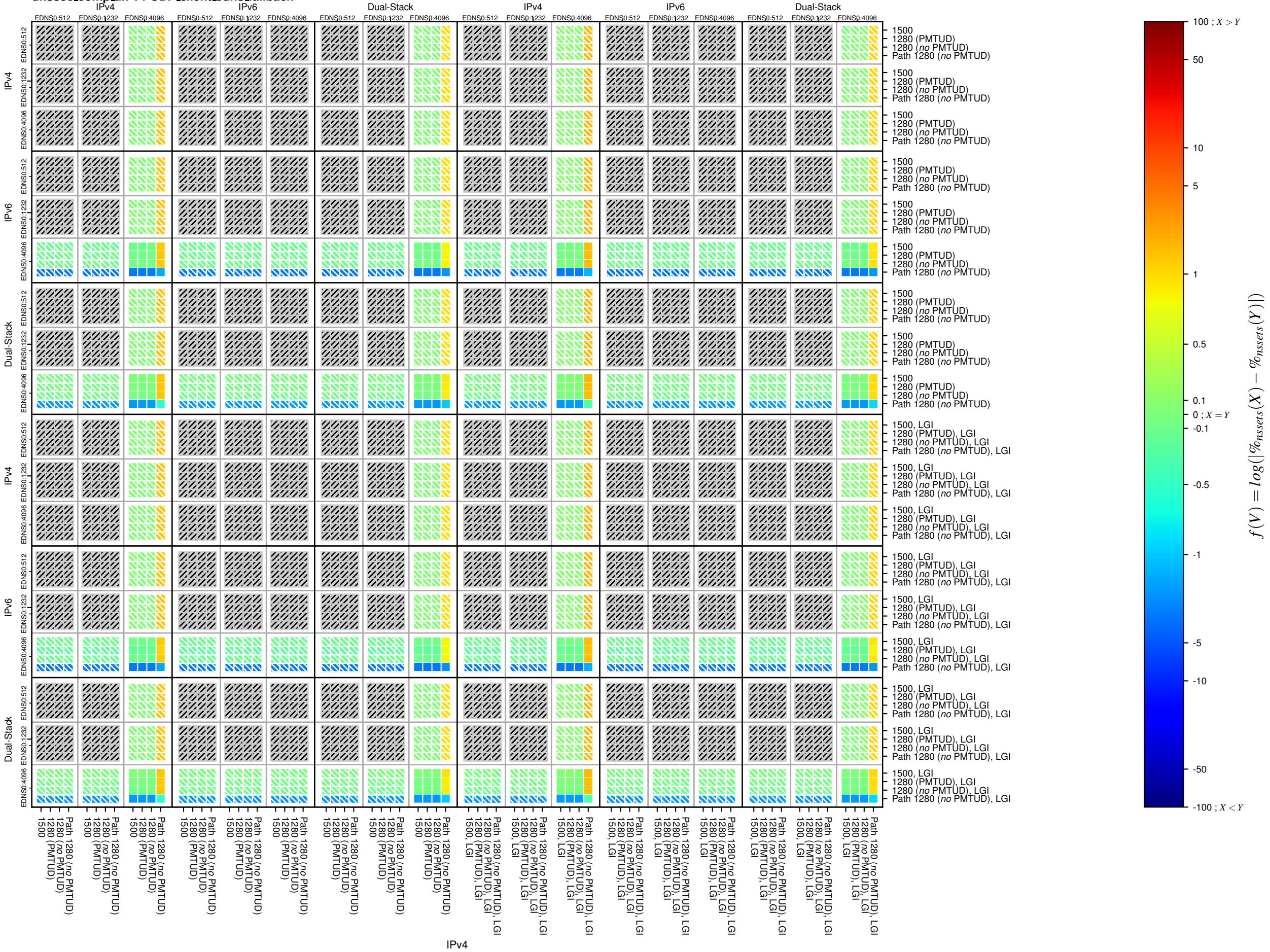
dnssec_comp_afv4-UDP_client_edns_fallback
