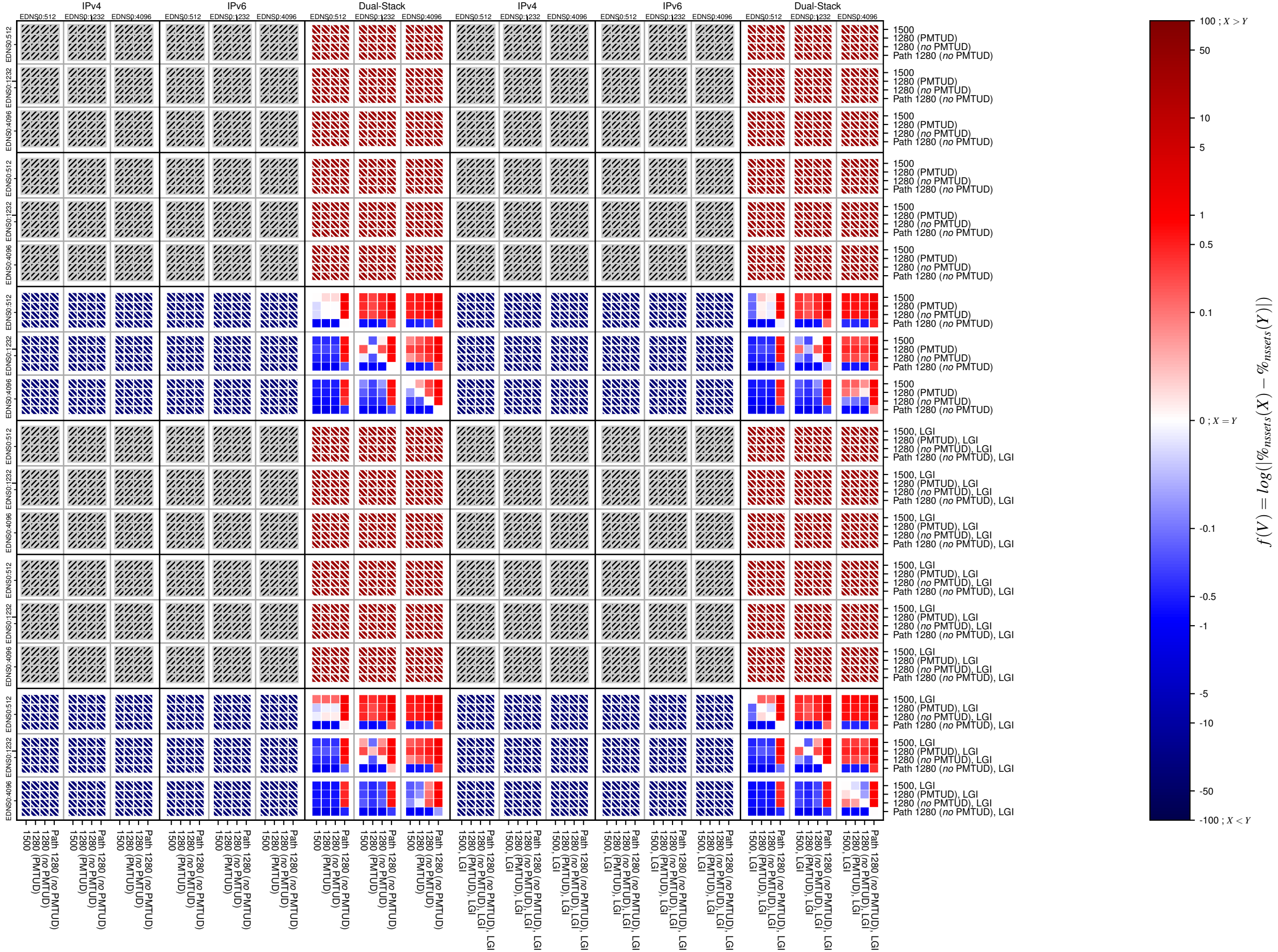
dnssec-v6-UDP_TCP_afc_count
