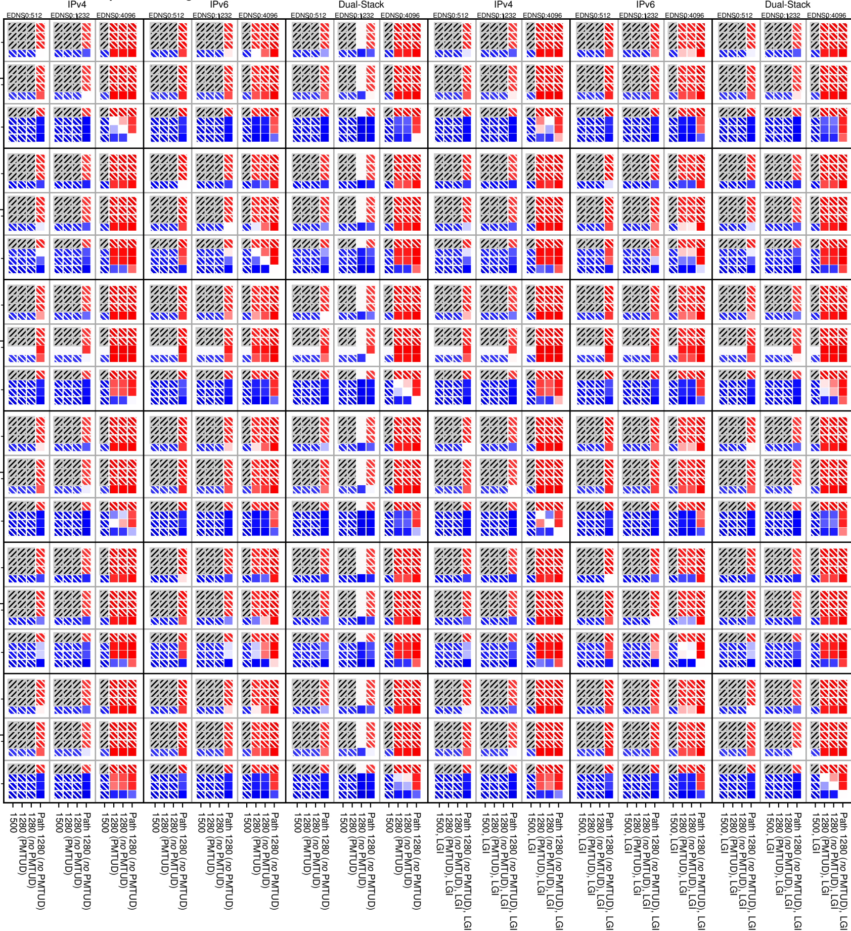
dnssec-both-UDP_packet_too_big
