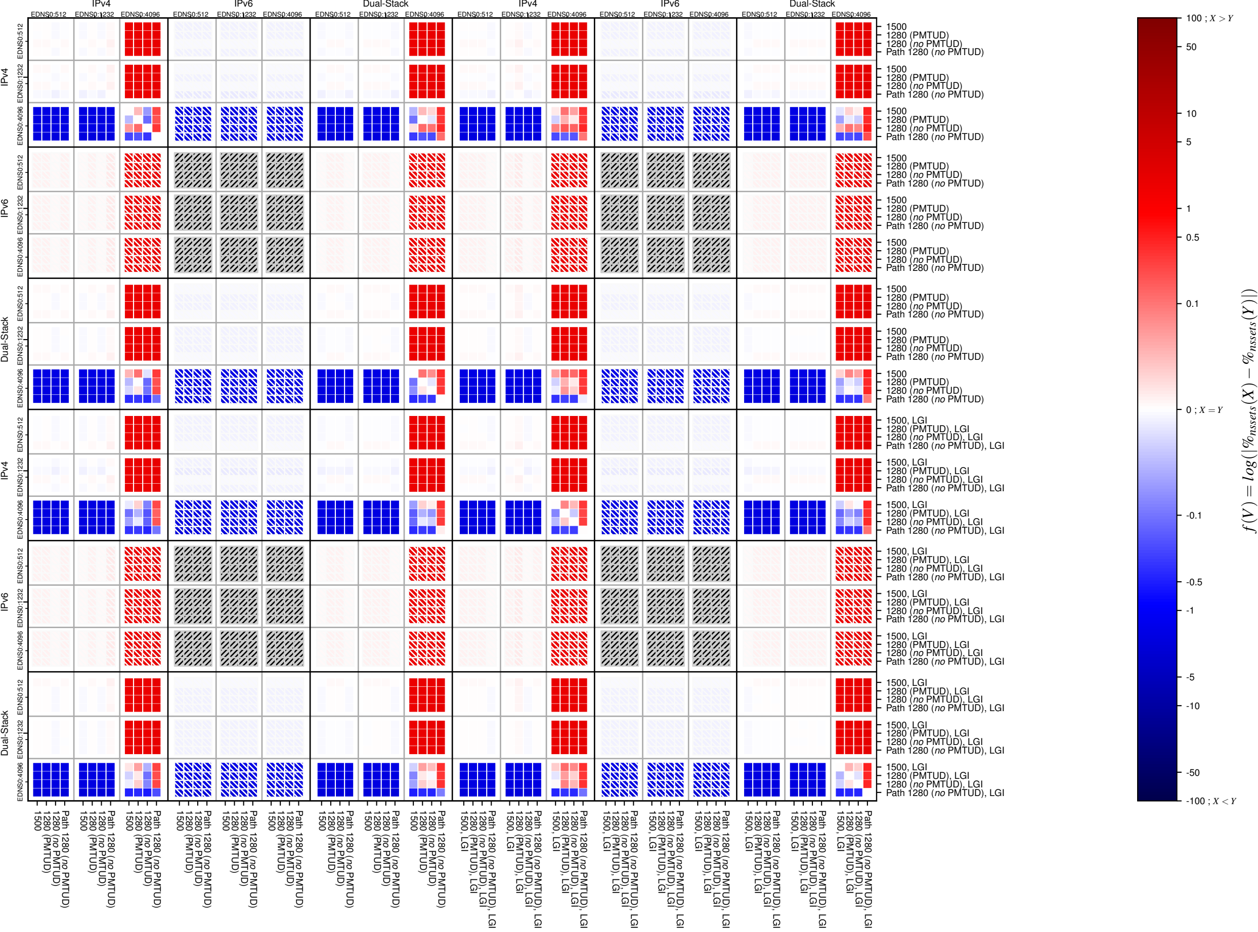
dnssec-v4-UDP_frag.too.big
