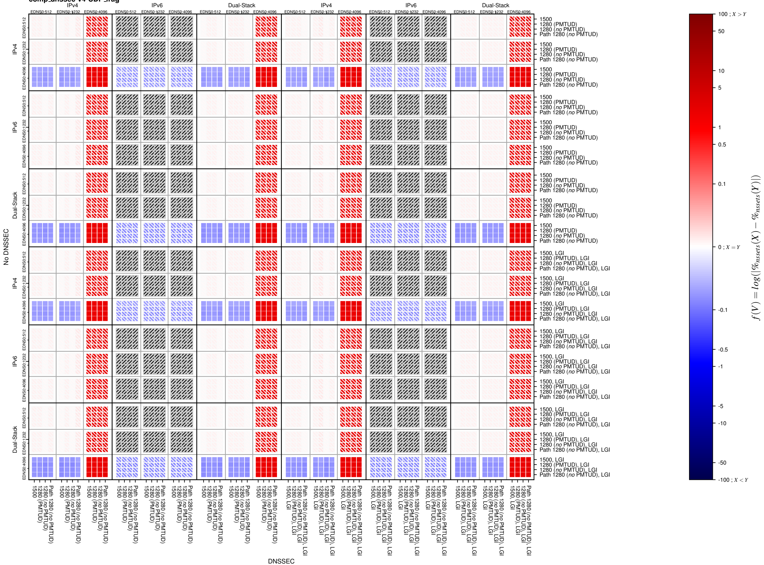
comp_dnsssec-v4-UDP_frag
