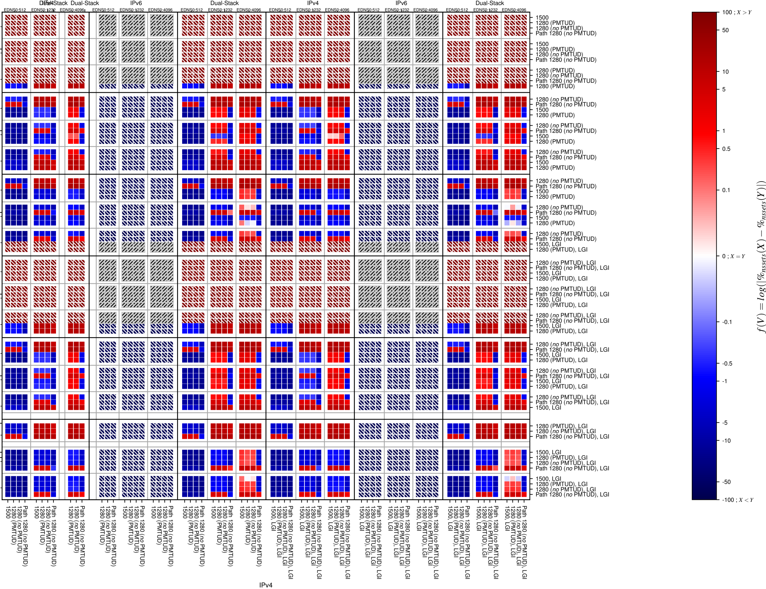
dnssec_comp_afi-v4-UDP_count
