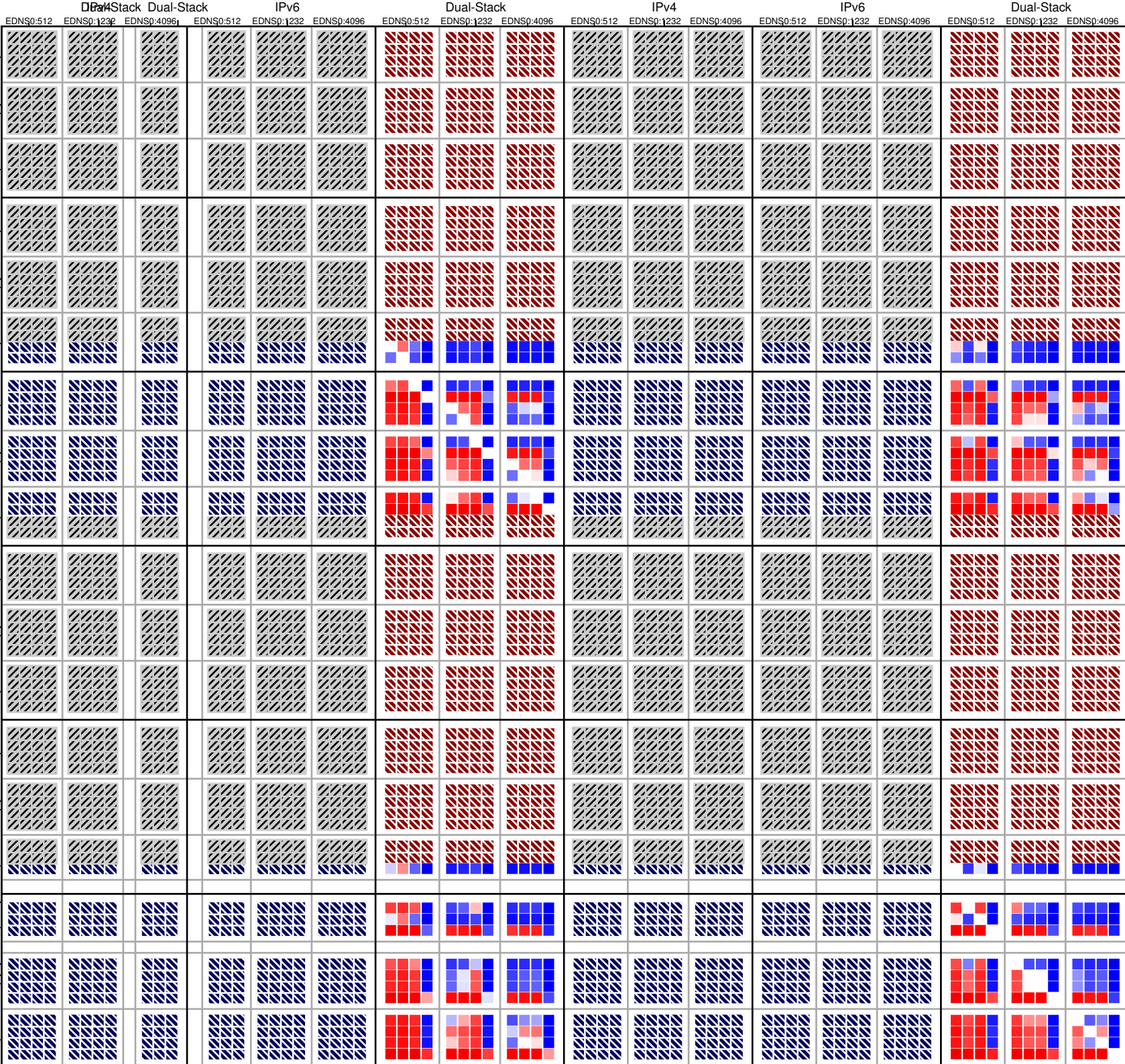
dnssec-v4-UDP.TCP.afs.count
