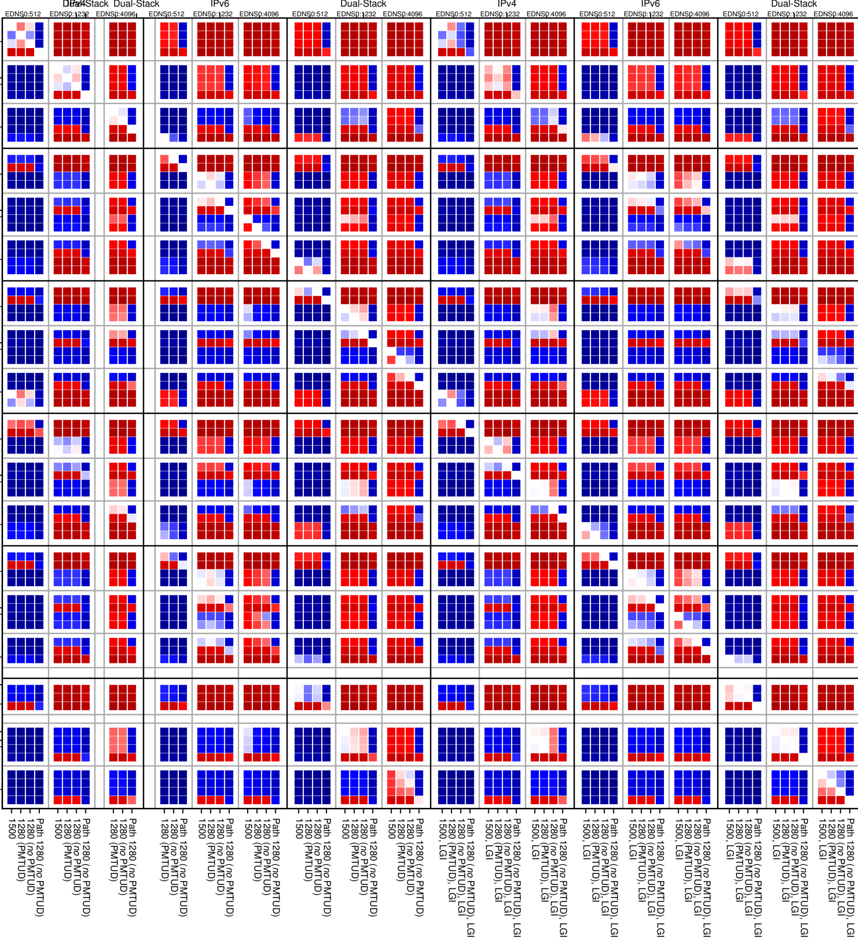
dnssec-both-UDP_count
