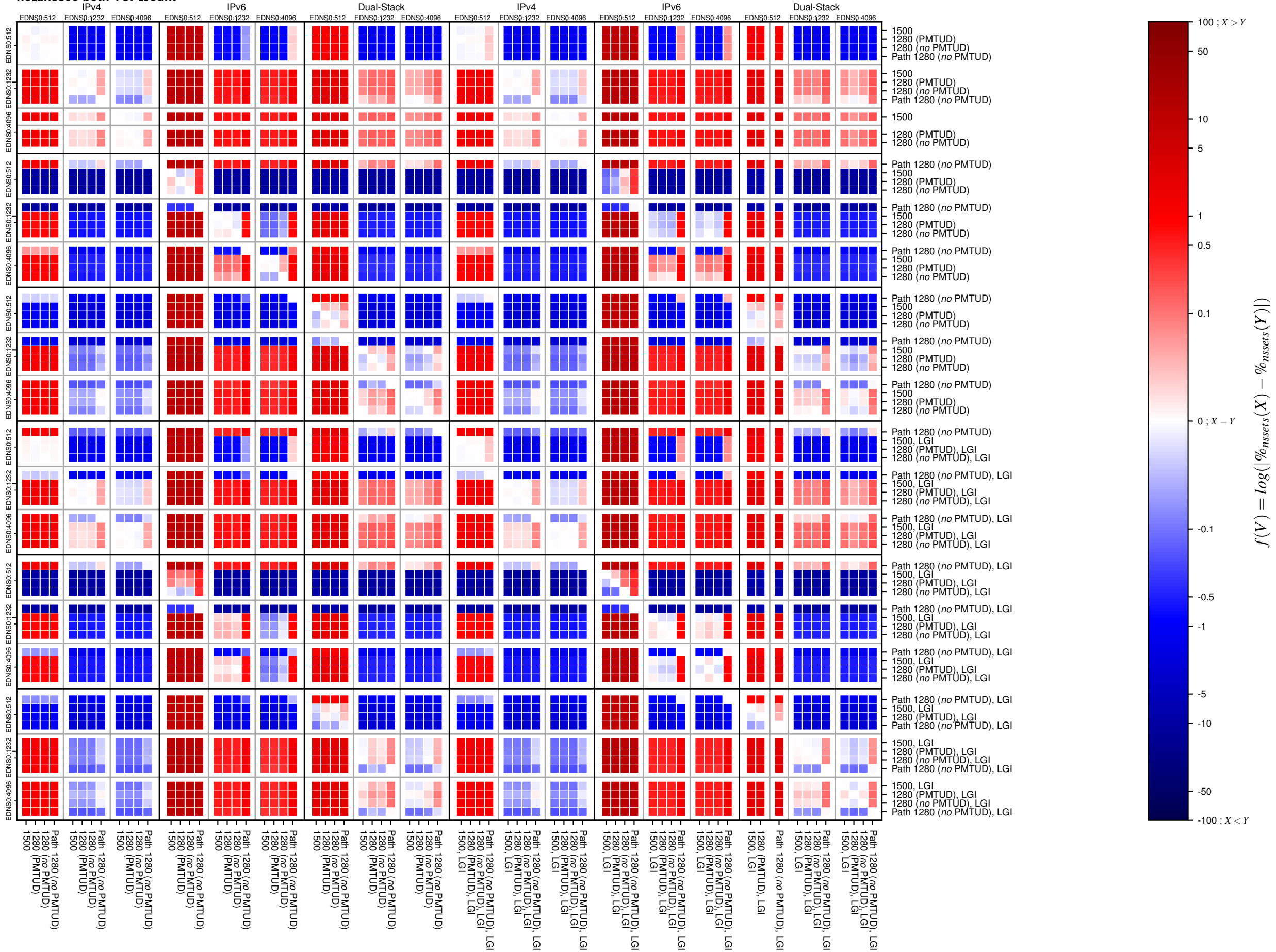
no_dnssec-both-TCP_count
