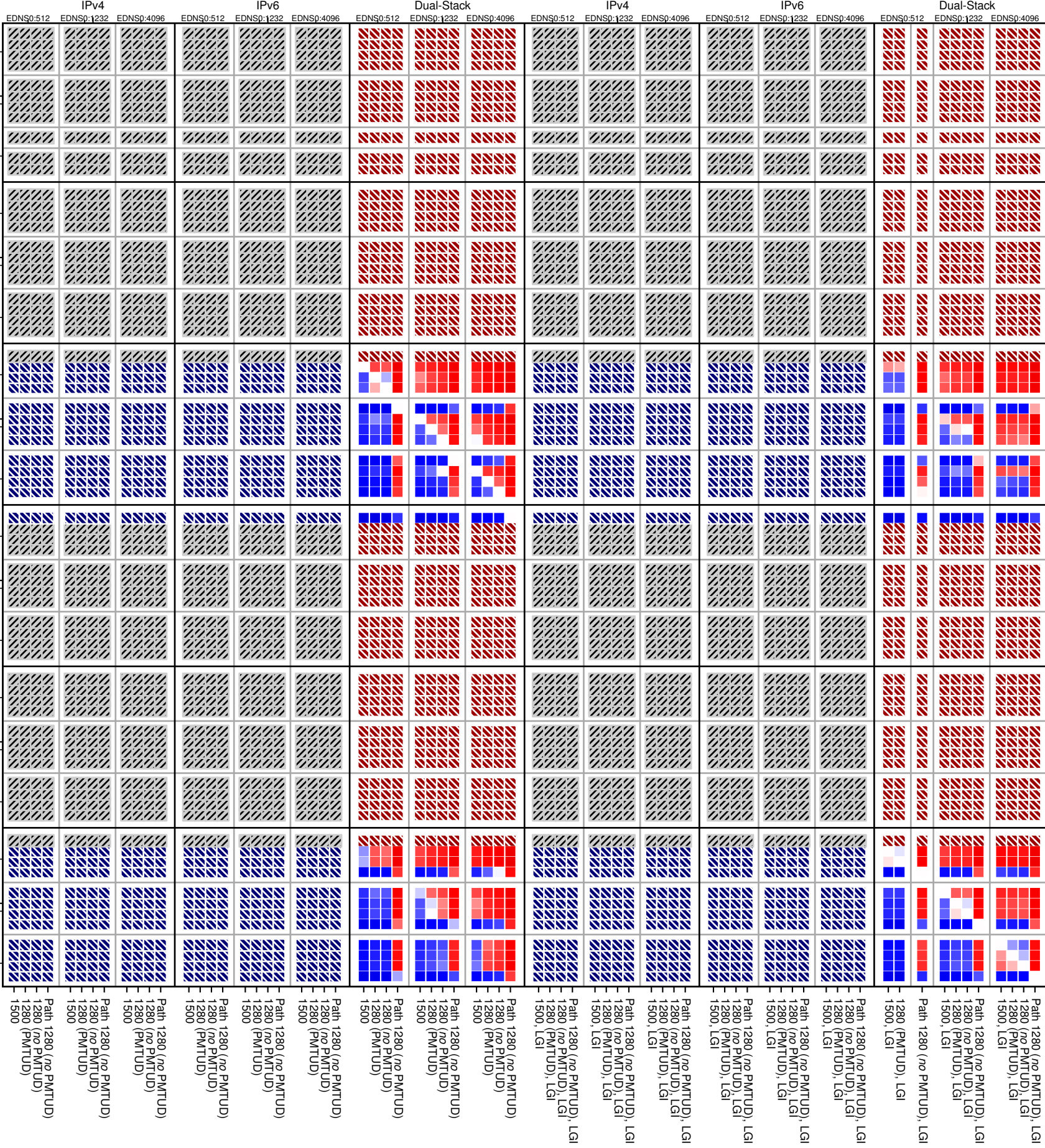
dnssec-v6-UDP_TCP_afi_count
