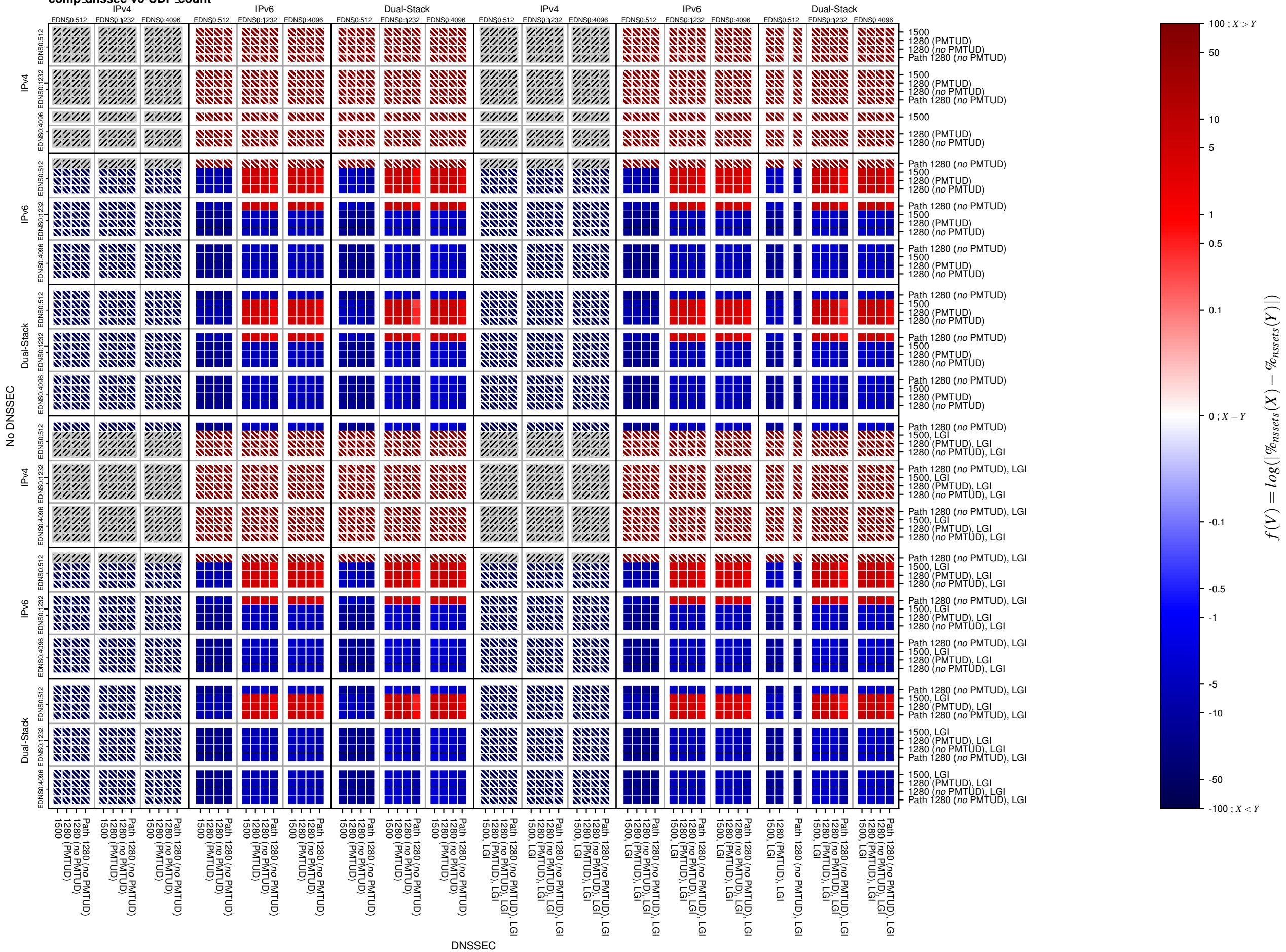
comp_dnssec-v6-UDP_count
